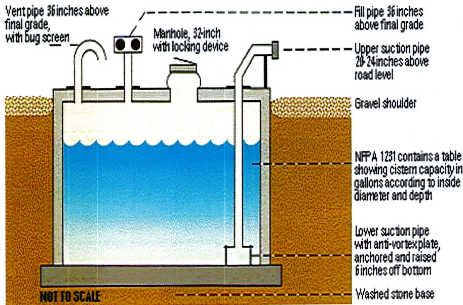
FIGURE B.5 Example of Construction of Water Cisterns Using an Underground Fiberglass Storage Tank.
